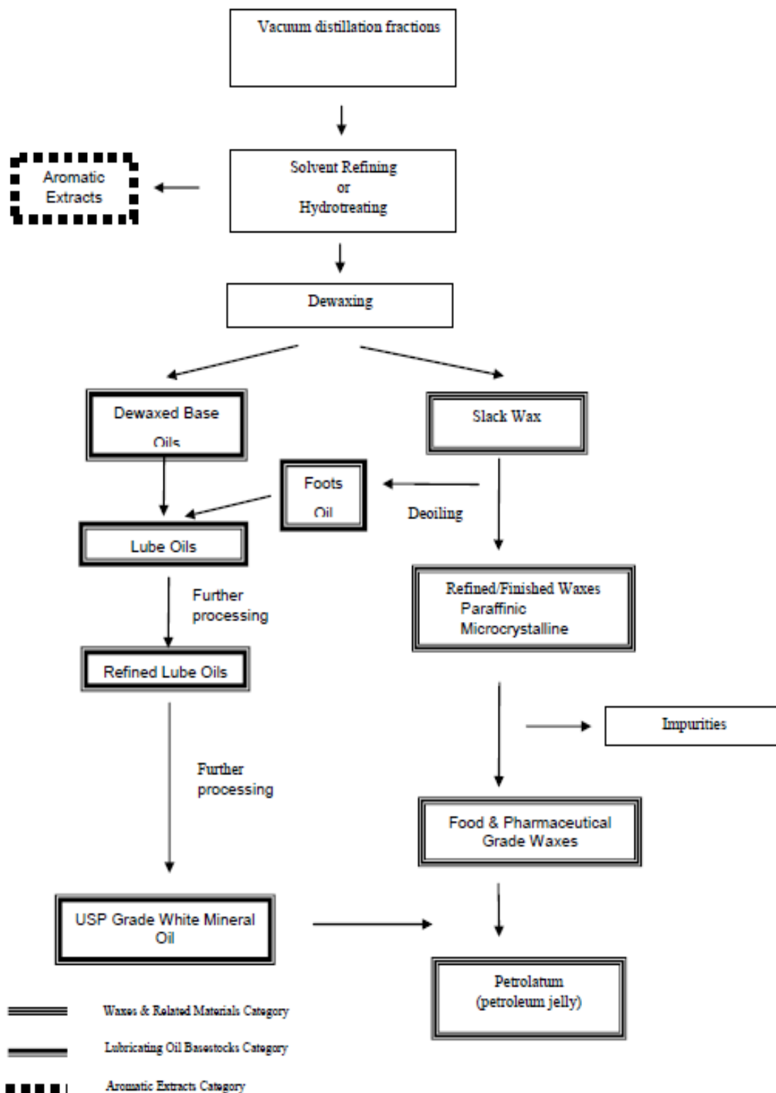
Figure 1. Schematic of the Production Process for Waxes and Related Materials
